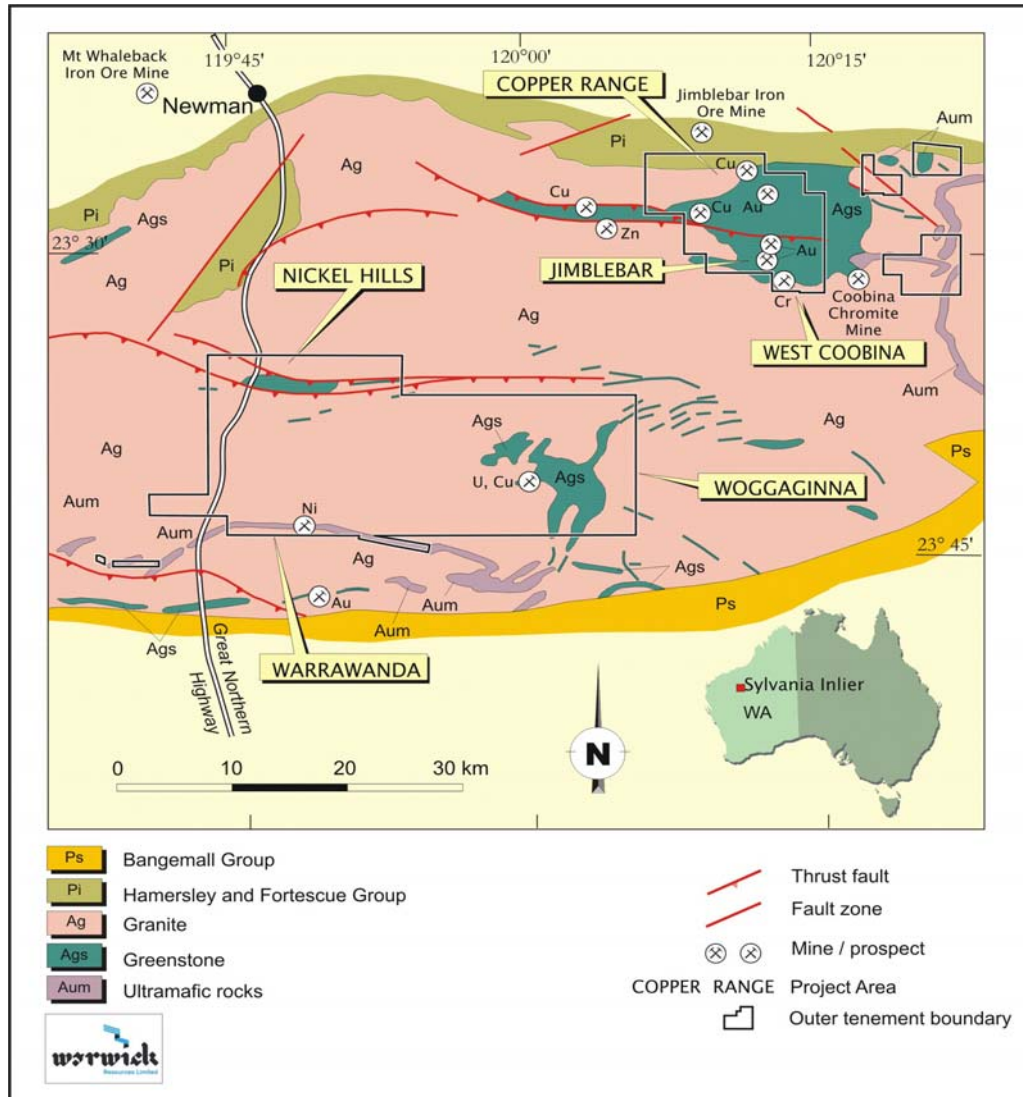
Geology of the Sylvania Inlier showing Projects
